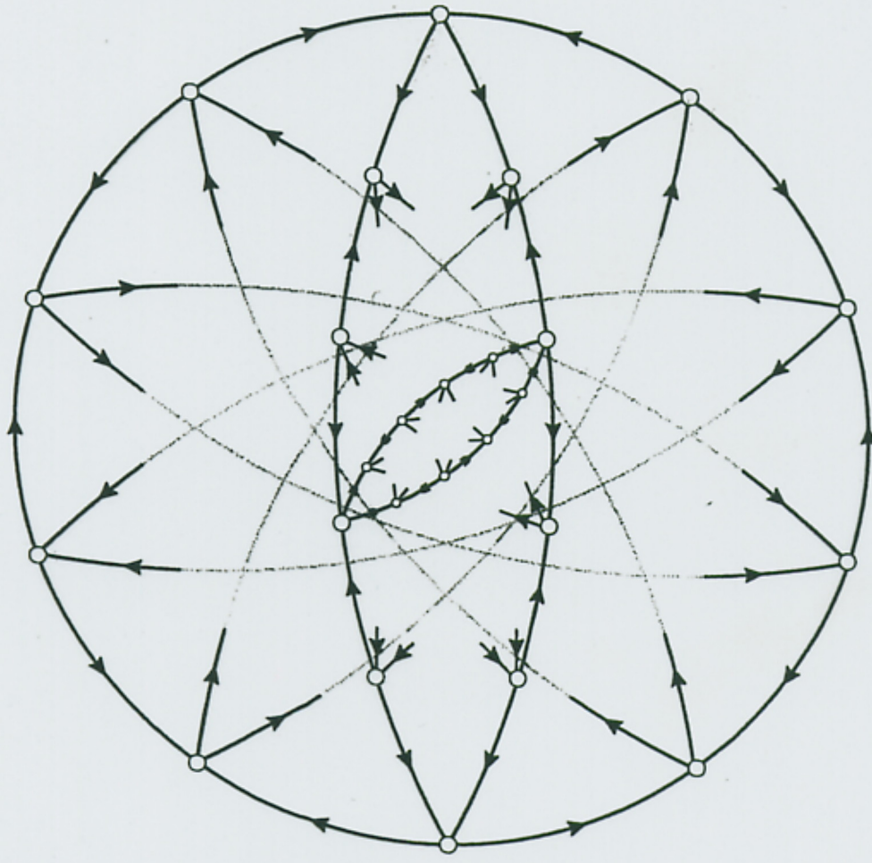
Figure 1: The construction of a highly arc-transitive digraph without property Z and having alternating cycles of length 2n , for n = 5 .
